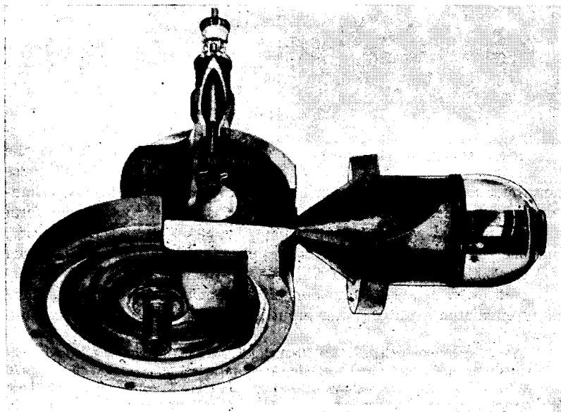
FIG. 19-23.—Cutaway view of 4J77 magnetron.
